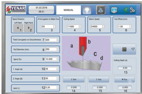
Grooving Control Screen
